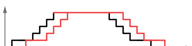
FIFO CCpp
