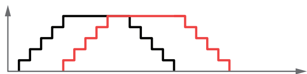
LIFO CCpp
