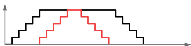
FIFO CCpp
